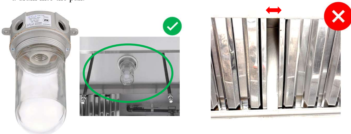
Figure 6. Your service-entry power supply shall have a male inlet, secured to the Food truck, in a weather rated casing or a direct connection to the breaker box. Never use a double male connection.
