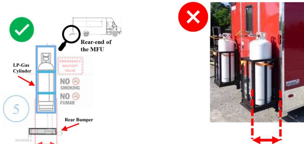
Figure 1. LP-Gas Cylinders must be protected from fall, car crashes or bystanders.
